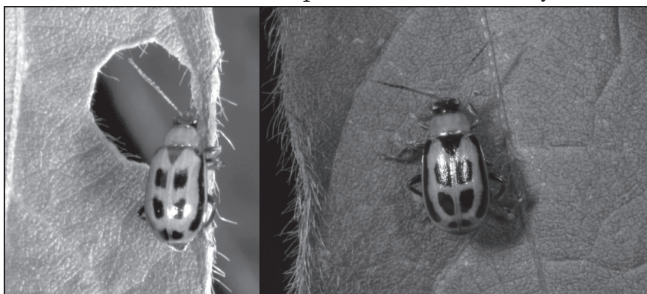
Figure 5. Both color forms of the bean leaf beetle, and characteristic round foliar feeding damage.
