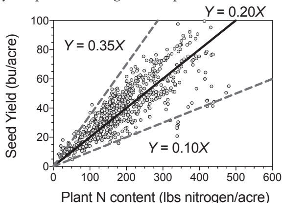
Figure 2. Relationship between seed yield and plant nitrogen content at maturity for soybean plant.
