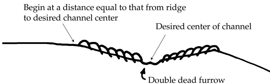
Figure 5. Enlarging and widening the terrace channel
