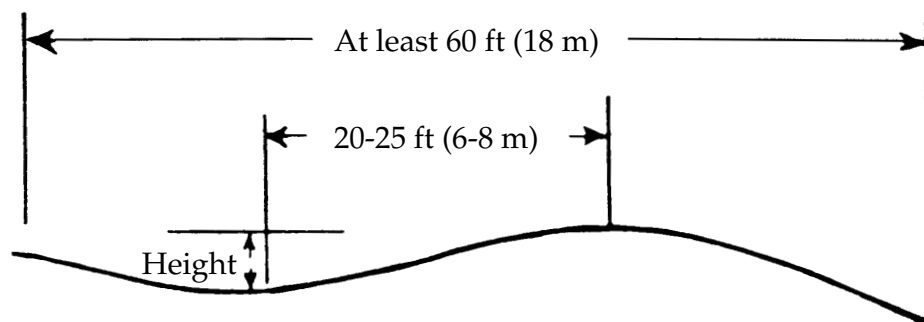
Figure 3. Wide, smooth terrace section recommended for crossing the terrace with equipment.
