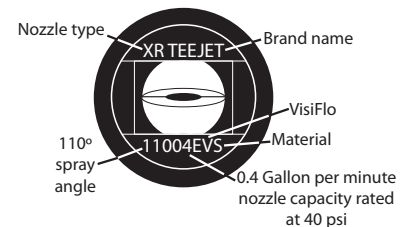
Calibration cup (8) and nozzle cleaning brush (9); Flat-fan nozzle nomenclature (10)
